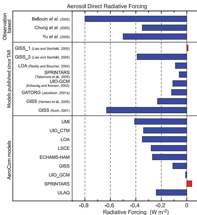
Figure 2.13. Estimates of the direct aerosol RF from observationally based studies, independent model studies, and AeroCom results with identical aerosol and aerosol precursor emissions. GISS_1 refers to a study employing an internal mixture of aerosol, and GISS_2 to a study employing an external mixture. See Table 2.4, Note (a) for descriptions of models.
